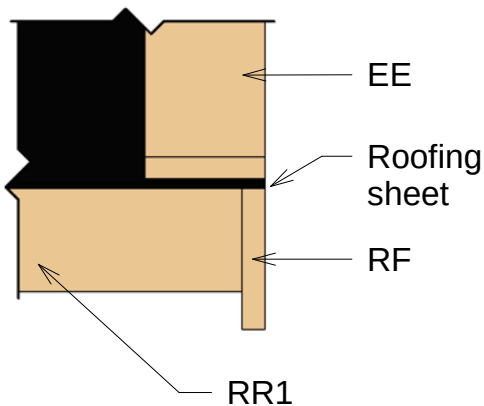
3 Roof Reinforcement
